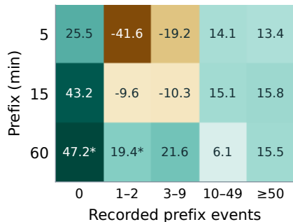
SEISMIC | Hurdle
