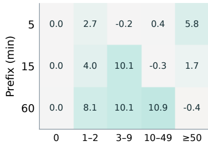
SEISMIC | Hurdle
