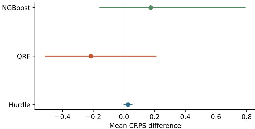
SEISMIC: noise minus I0
