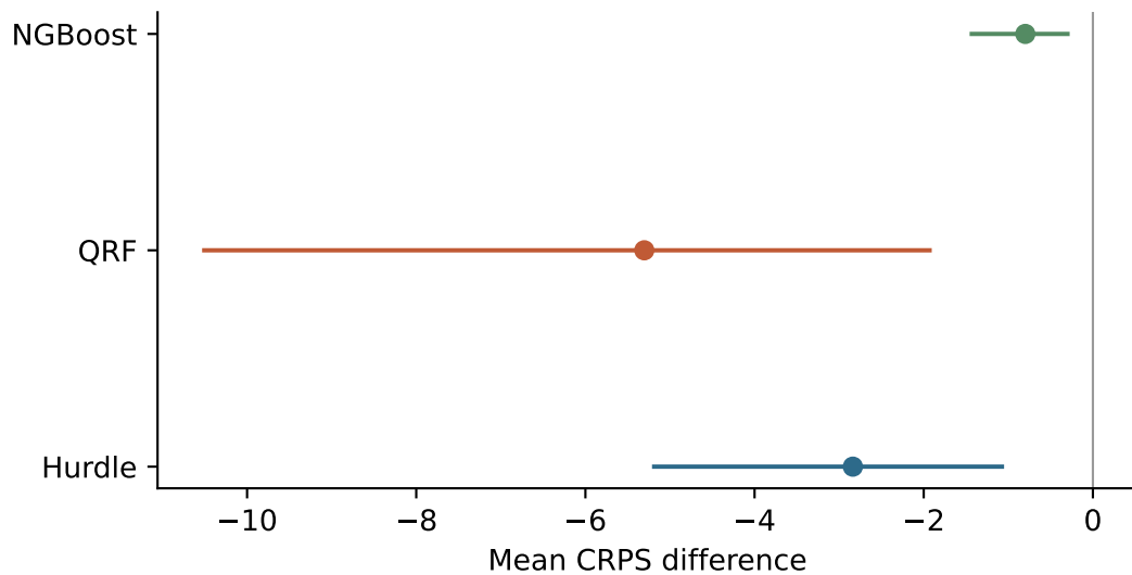
SEISMIC: I1 minus noise
