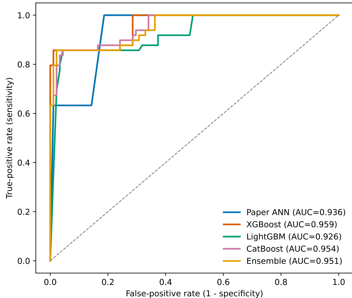
External validation ROC curves
