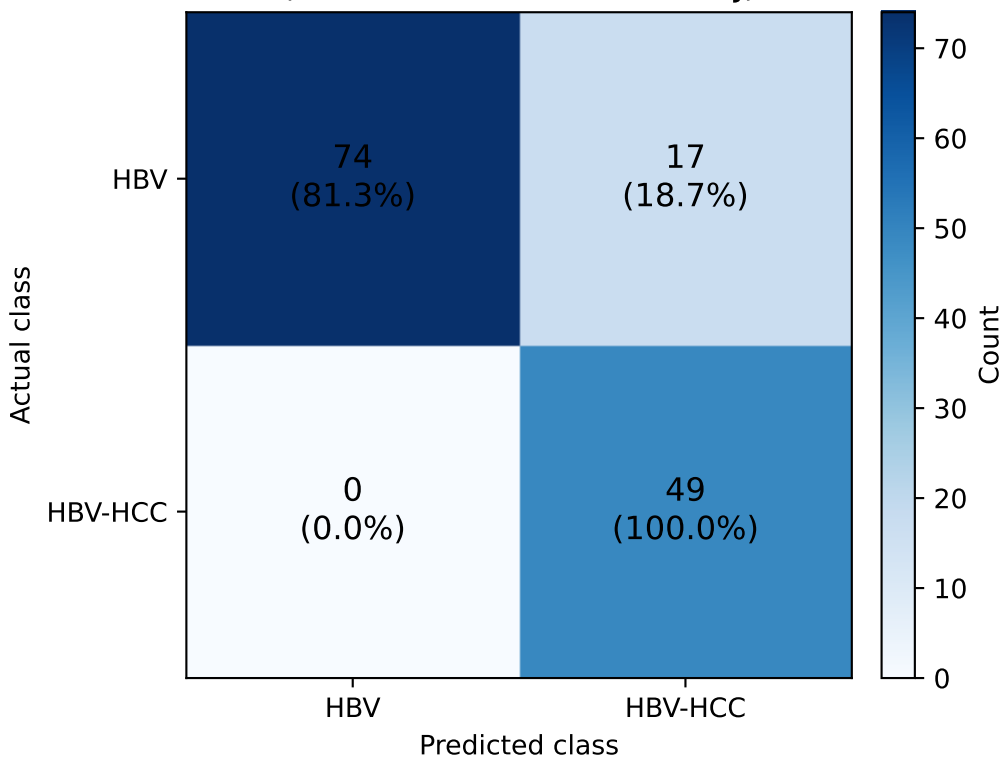
Paper ANN: validation confusion matrix (threshold=0.886, Youden's J)
