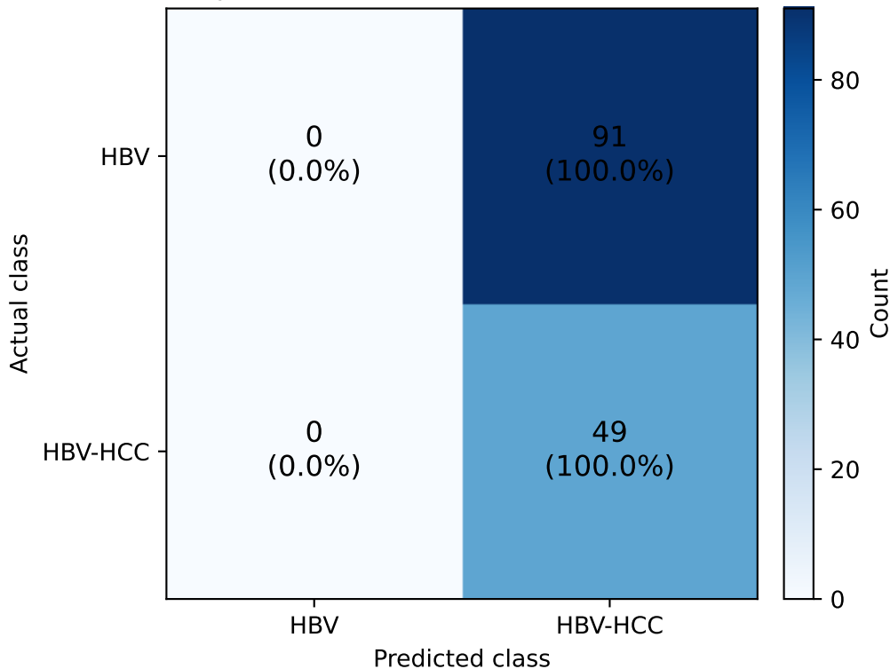
Paper ANN: validation confusion matrix
