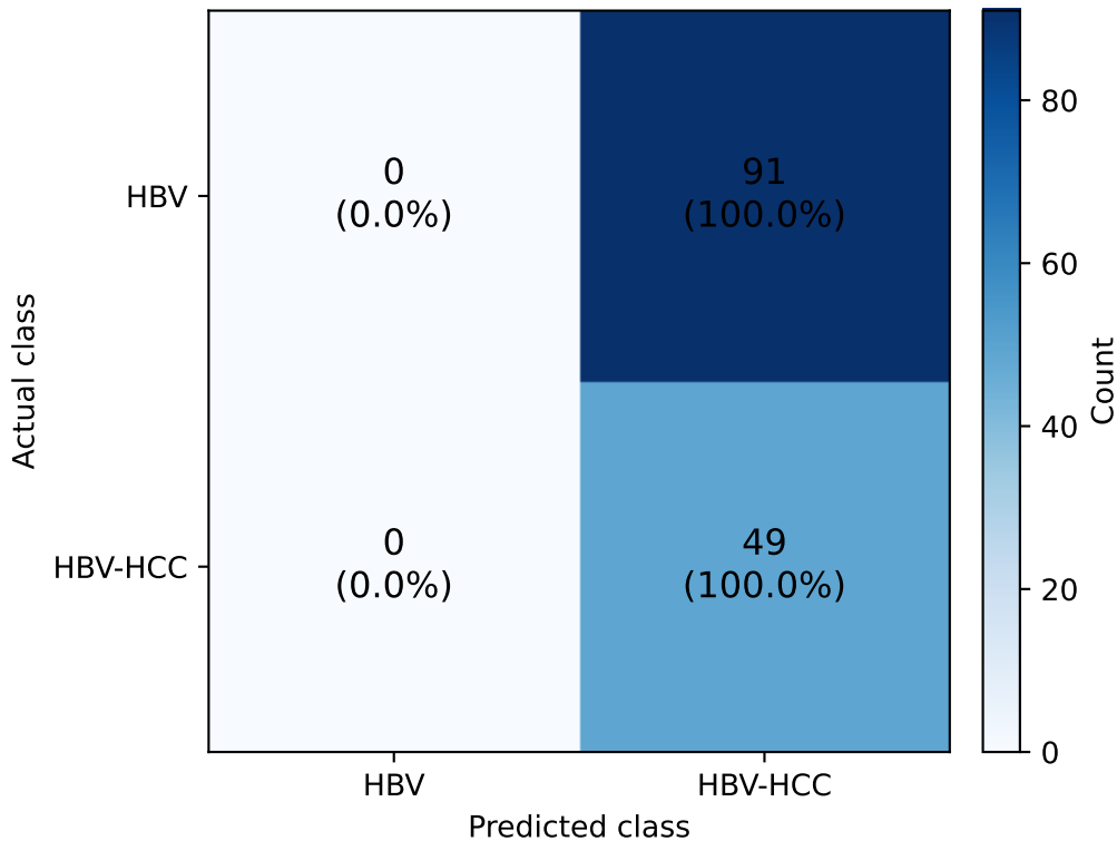
Ensemble: validation confusion matrix
