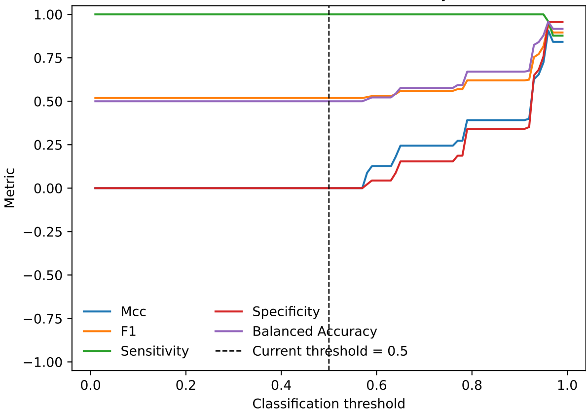
Ensemble threshold sensitivity
