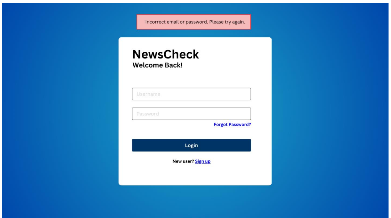
Figure 3.11 Incorrect Login
