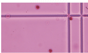
Brightfield Leukocyte
