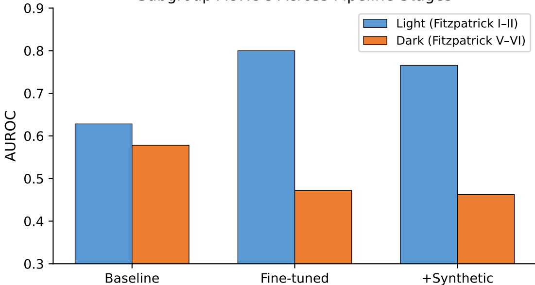
Subgroup AUROC Across Pipeline Stages
