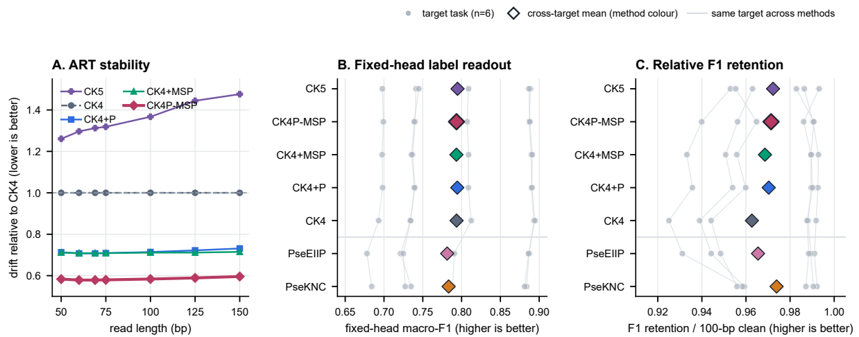
Figure 4 External probes separate simulator stability from coarse fixed-head label retention. (A) Standardized L2 drift relative to CK4 at each ART read length; the horizontal CK4 reference is 1.0 and lower ratios indicate less within-length drift. The ART layer contains 55,961 matched clean/simulated pairs across 50, 60, 69, 75, 100, 125 and 150 bp. Lines are descriptive length-specific ratios without uncertainty intervals; the selected ART cycle profile produces a non-monotonic error load. (B) Target-level mean macro-F1 across eight shifted CAMI_TOY_low length-by-condition cells. A class-balanced logistic head was trained only on 100-bp clean sources and reused without refitting. The endpoint comprises six source-grouped target-versus-background probes and is not a fine-grained multi-class taxonomy benchmark. (C) Macro-F1 retention relative to each method's own 100-bp clean baseline. Panels B and C contain six prespecified one-versus-background tasks with 1,200 target and 1,200 background source groups each. Neutral circles denote target-task estimates, method-coloured diamonds denote cross-target means and faint lines preserve target pairing across methods. The six tasks share one CAMI source pool, so cross-target summaries describe task-level consistency.
