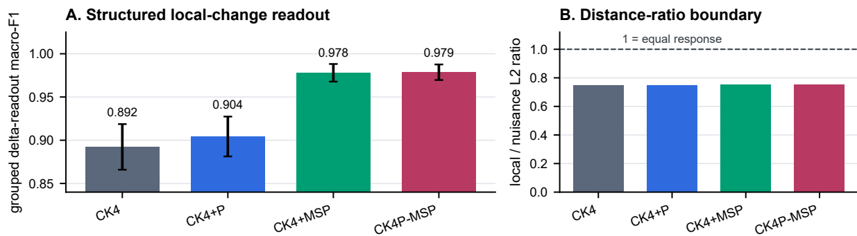
Figure 6 Common template-grouped local-change readout and distance-ratio boundary across 12 length-by-local-mode cells (250 template triplets per cell). (A) Mean local-versus-nuisance macro-F1 under template-grouped fivefold cross-validation shows that MSP accounts for most of the compact local-change readout increment. (B) CK4P-MSP and CK4 have similar mean local-to-nuisance L2 ratios, whereas full-position and property-channel representations provide stronger distance amplification. Error bars are 95% matched-cell bootstrap intervals; they quantify variation across the controlled grid, for which independent biological-cohort variation was not sampled. Higher values indicate greater readout or distance selectivity, respectively.
