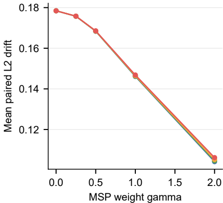
69 bp stability
