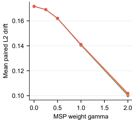
75 bp stability
