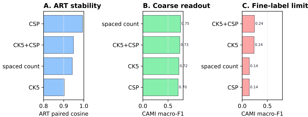
Figure 4 ART stability and CAMI coarse/fine readout probes. Alt text: Three-panel comparison of ART stability and CAMI coarse and fine readout probes, highlighting stable external behavior and limited fine-label readability.
