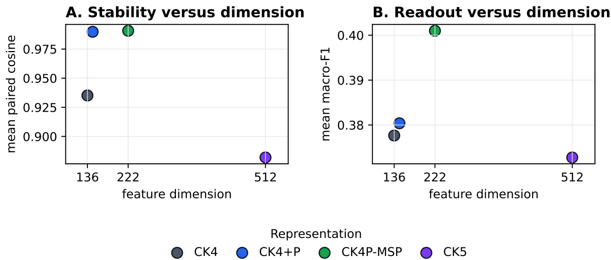
Figure 3 CK4P-MSP stability-readout-dimension trade-off. Alt text: Scatter plots showing CK4P-MSP among compact representations in the stability, readout and dimension trade-off space.
