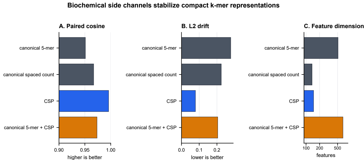
Figure 2 Compact stability under controlled perturbation.
