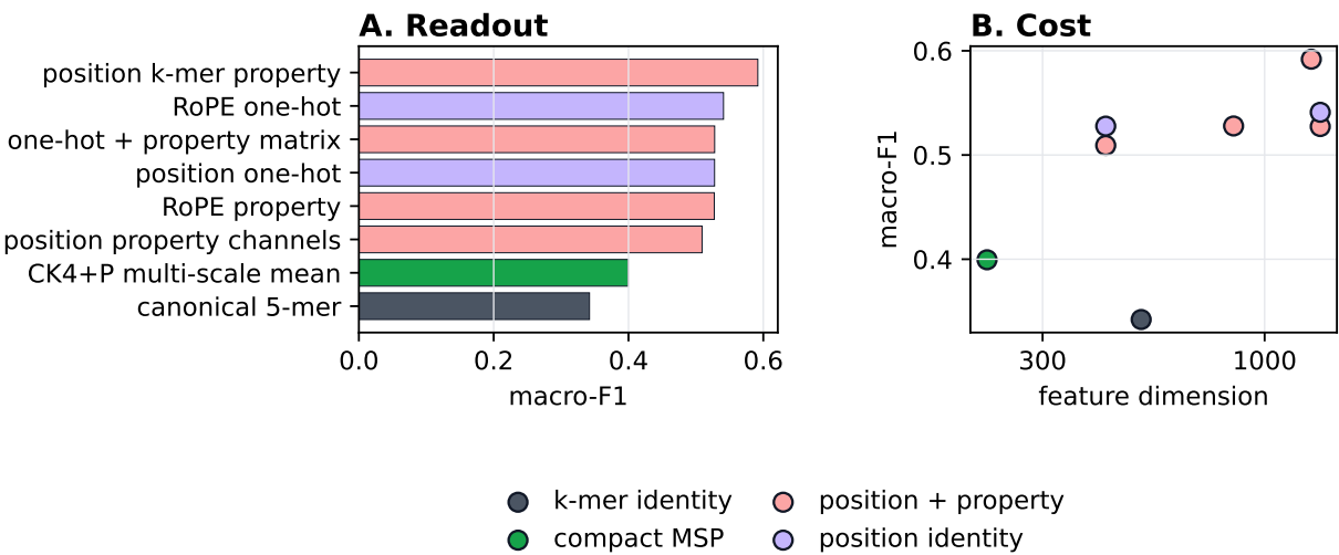
Figure 5 Full-position diagnostic upper bound for positional information. Alt text: Bar and scatter plots showing that full-position matrices add positional readout value at substantially higher feature dimension.
