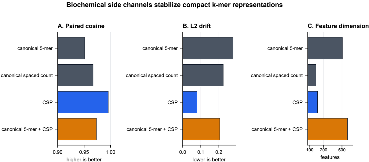
Figure 2 Compact stability under controlled perturbation. Alt text: Bar plots comparing paired cosine, L2 drift and feature dimension across compact k-mer, biochemical and spaced-property representations.
