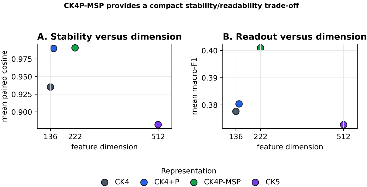
Figure 3 CK4P-MSP stability-readout-dimension trade-off. Alt text: Scatter plots showing CK4P-MSP among compact representations in the stability, readout and dimension trade-off space.
