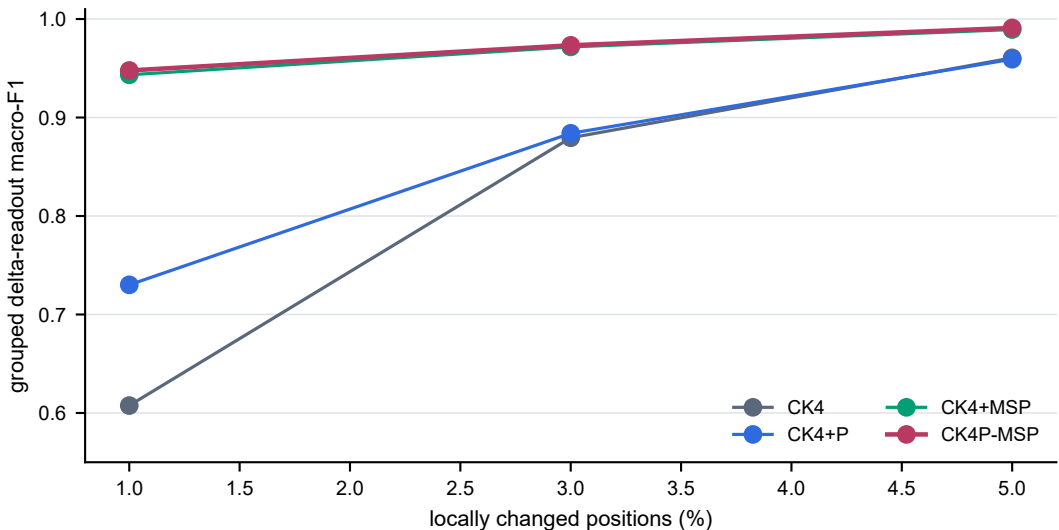
S4. MSP-associated readability persists across effect sizes
