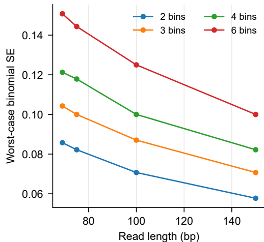
D. Short-bin sampling bound
