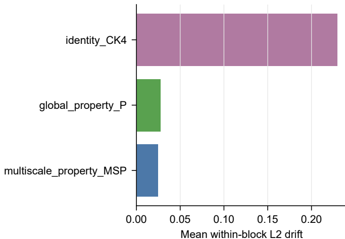
C. Drift decomposed by block
