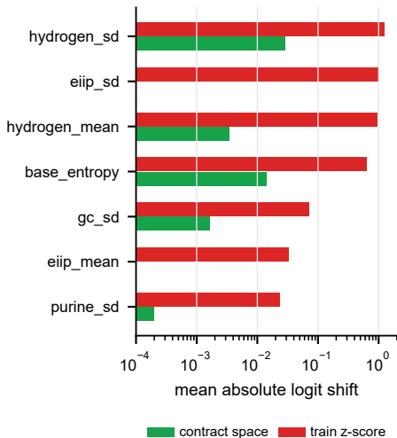
B. N-mask coordinate effect
