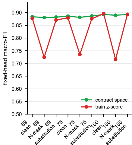
A. Preprocessing boundary
