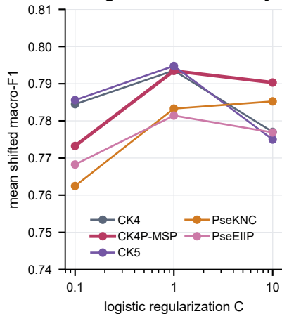
C. Regularization sensitivity
