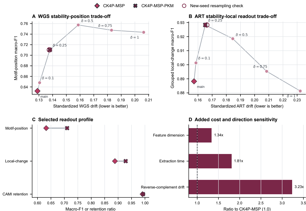
Figure S15 Exploratory CK4P-MSP-PKM positional-readability Pareto audit. (A) The prespecified PKM weight path compares mean WGS standardized drift across 24 length-by-perturbation cells with motif-position macro-F1; lower drift and higher readout are preferable. (B) The same path compares mean ART drift across seven read lengths with template-grouped local-change macro-F1; lower drift and higher readout are preferable. Diamonds mark CK4P-MSP, crosses mark the selected CK4P-MSP-PKM point at \delta = 0.25 , and open circles mark the new-seed resampling check. The resampling check reuses the benchmark resources and is not an independent external replication. (C) Dumbbells compare the two methods on motif-position macro-F1, grouped local-change macro-F1 and CAMI fixed-head retention. (D) Bars report the CK4P-MSP-PKM-to-CK4P-MSP ratios for feature dimension, median reference extraction time over two actual 10,000-read batches, and mean reverse-complement-pair drift over 5,000 pairs; values above one indicate added cost or direction sensitivity. CK4P-MSP-PKM increased the two structured readouts but also increased drift, dimension, runtime and input-direction sensitivity. It is a supplementary Pareto extension, not a generally superior replacement for CK4P-MSP.
