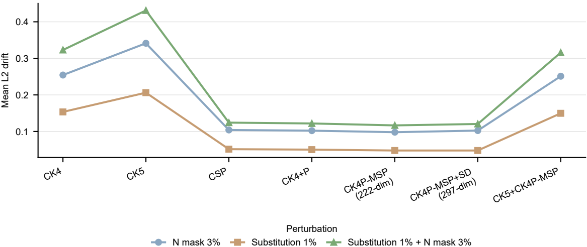
Supplementary Figure S10 | CAMI II marine subset probe n=4,000 reads; 48,000 length/condition rows; unlabeled perturbation-stability probe
