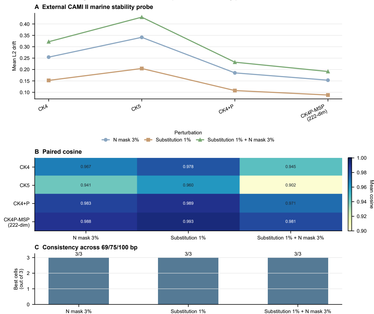
Supplementary Figure S10 | CAMI II marine subset probe n=4,000 reads; 48,000 length/condition rows; unlabeled perturbation-stability probe
