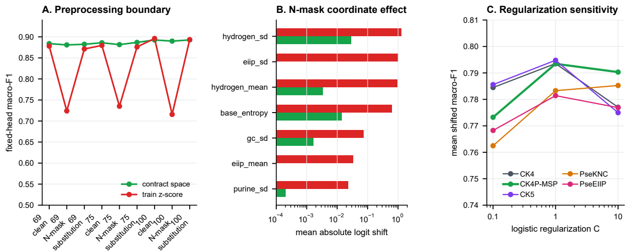
Figure S14 Frozen-head preprocessing and regularization sensitivity. (A) Macro-F1 for CK4P-MSP in the prespecified single CAMI target task. Contract-space probes use the declared row/block-normalized representation directly; train z-score probes apply coordinate-wise means and variances fitted only on the 100-bp clean training fold. Each point aggregates 2,486 held-out source groups through fivefold source-grouped cross-validation. (B) Mean absolute logistic-logit shifts of the seven most affected P coordinates under 100-bp, 3% N masking, averaged over five folds. The log axis contrasts contract-space contributions with amplification after train-fit z-scoring. (C) Mean shifted macro-F1 across six CAMI target tasks and eight non-baseline length-by-condition cells per target at C = 0.1, 1 and 10 . The classifier was otherwise unchanged and was never refitted on shifted conditions. C = 1 was prespecified; the other values are sensitivity analyses rather than selected alternatives. These panels show that low representation drift does not guarantee invariance to learned downstream preprocessing.
