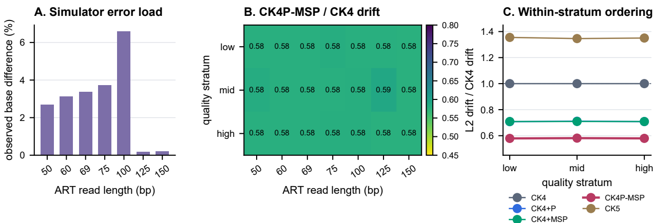
Figure S3 Current-contract ART error-load and quality-stratification audit using 55,961 matched clean/simulated pairs, represented as 111,922 rows, at 50, 60, 69, 75, 100, 125 and 150 bp. (A) Bars show the observed same-coordinate base-difference rate at each length; this descriptive mismatch rate is not an alignment-aware edit distance. (B) Heatmap cells show CK4P-MSP standardized L2 drift divided by CK4 drift within each length and low-, middle- or high-quality stratum; values below one indicate less drift than CK4. (C) Lines show mean within-stratum drift ratios for CK4, CK4+P, CK4+MSP, CK4P-MSP and CK5, averaged over the seven lengths. Panels report descriptive means without uncertainty intervals. Because the selected ART cycle profile produces a non-monotonic error load across lengths, the figure supports within-length and within-stratum ordering rather than a causal read-length trend.
