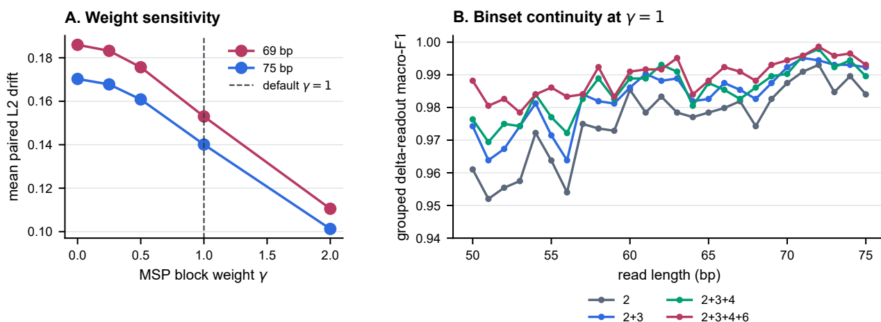
Figure S6 MSP binset and weight-sensitivity audit. (A) Points are mean drift without uncertainty intervals over the prespecified WGS perturbations at 69 and 75 bp for the complete 2+3+4+6 binset and \gamma \in \{0, 0.25, 0.5, 1, 2\} ; lower is preferable. (B) Lines are mean grouped delta-readout macro-F1 over four local modes at every integer length from 50 to 75 bp, using 180 template triplets per length-by-mode cell at \gamma = 1 for cumulative binsets 2, 2+3, 2+3+4 and 2+3+4+6; higher is preferable. All derivatives of one template were retained in the same fold during fivefold grouped cross-validation. No uncertainty intervals are shown. The audit tests sensitivity rather than selecting an optimal binset or weight.
