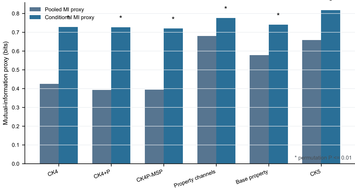
Supplementary Figure S2 | Empirical MI proxy audit
