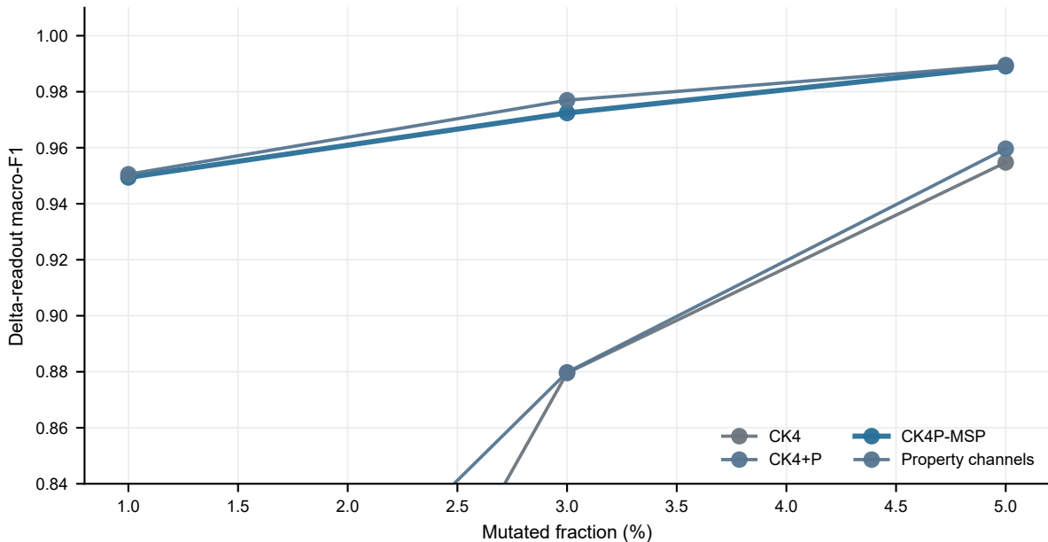
Supplementary Figure S4 | Local-mutation fraction sensitivity
