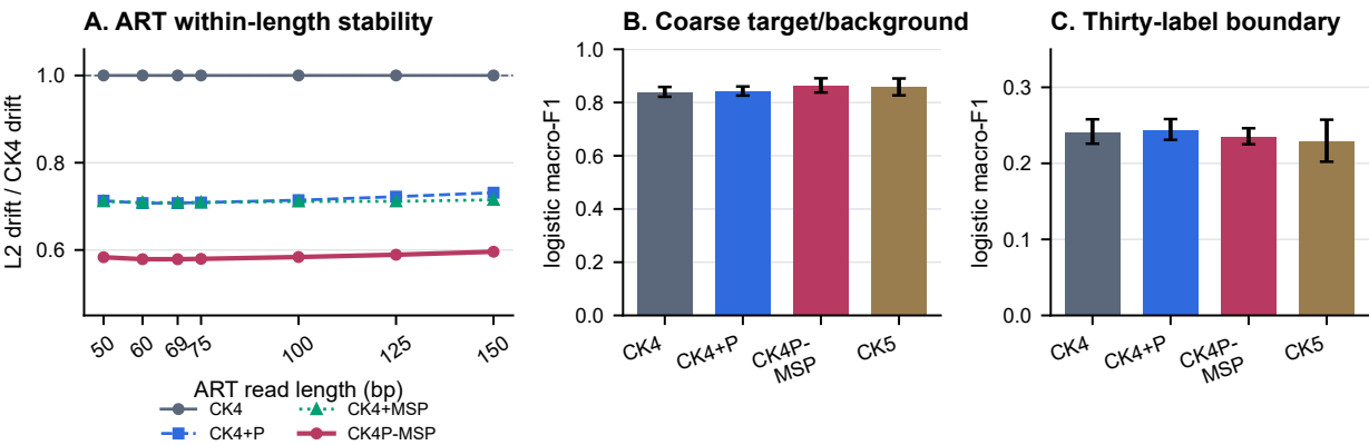
Figure 4 Current-contract external probes separate simulator stability from task-limited readability. (A) Standardized L2 drift relative to CK4 at each ART read length; the horizontal CK4 reference is 1.0 and lower ratios indicate less within-length drift. The ART layer contains 55,961 matched clean/simulated pairs across 50, 60, 69, 75, 100, 125 and 150 bp. Lines are descriptive length-specific ratios without uncertainty intervals and are not interpreted as a monotonic physical length response. (B) Mean logistic macro-F1 across nine CAMI_TOY_low length-by-condition cells for binary target-versus-background readout. (C) The corresponding 30-label probe, in which all compact representations remain weak and CK4P-MSP does not lead. Higher macro-F1 is preferable in panels B and C. Error bars are 95% bootstrap intervals across analysis cells and do not represent independent-community confidence intervals. Both CAMI_TOY panels use current-contract features from 24,000 labelled source reads expanded to 216,000 rows.
