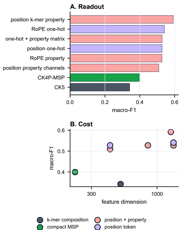
Figure 5 Full-position diagnostic upper bound for positional information. (A) Macro-F1 on controlled positional readout tasks compares compact summaries with representations that retain per-position token or property channels. (B) Readout is plotted against feature dimension to show the cost of preserving near-explicit positional information. CK4P-MSP provides a compact coarse summary and is not the positional-readout upper bound.
