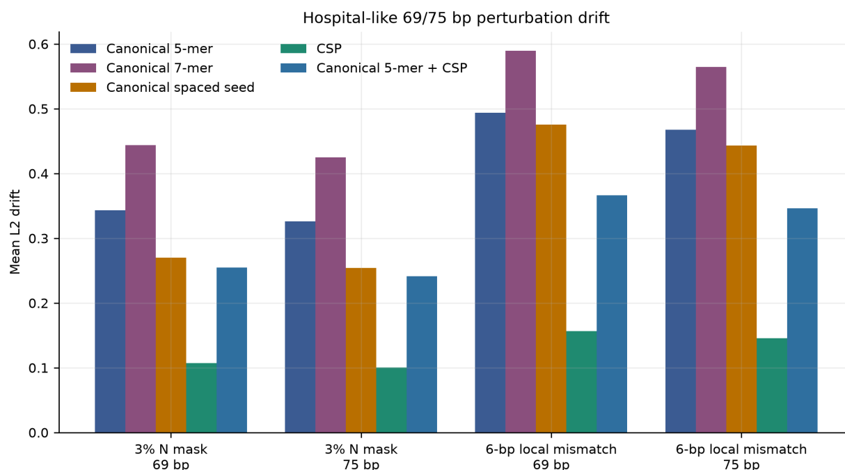
Figure 2: Hospital-like 69/75 bp perturbation drift.
