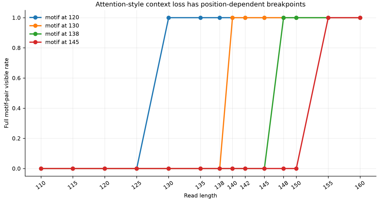
Figure 6: Attention-style context visibility breakpoints.
