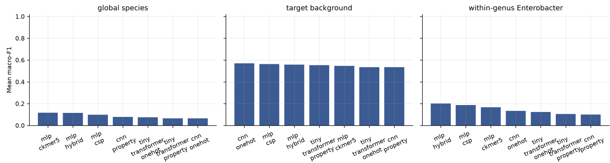
Figure 5: Deterministic neural compatibility probes.
