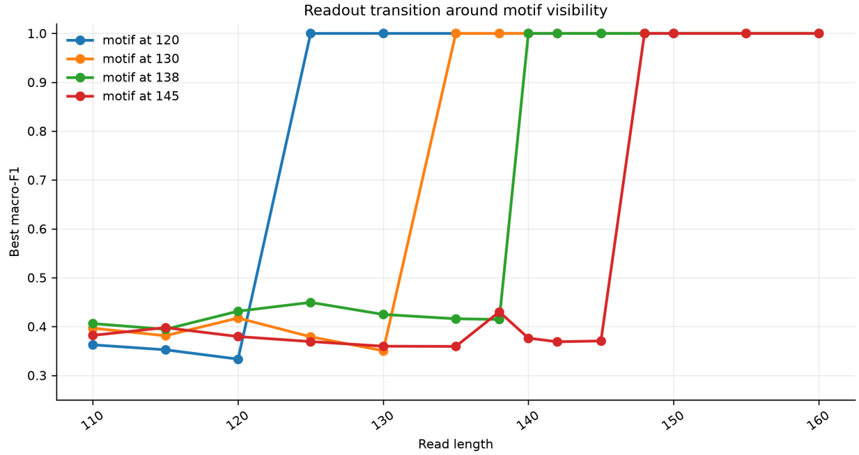
Figure 7: Best readout transitions around motif visibility.
