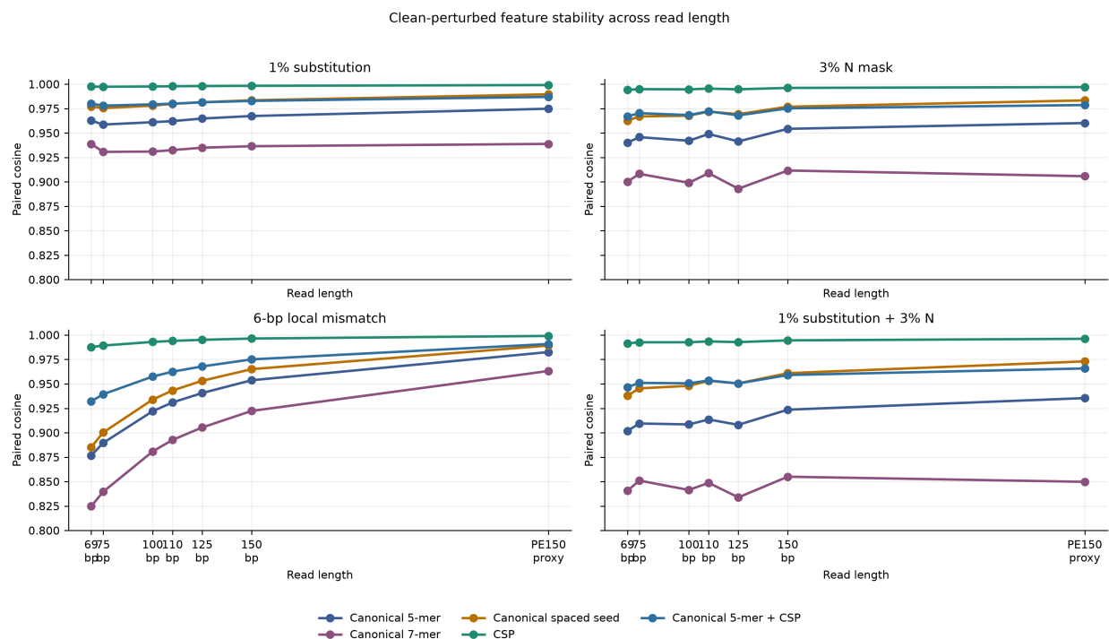
Figure 1: Clean-perturbed feature stability across read length.
