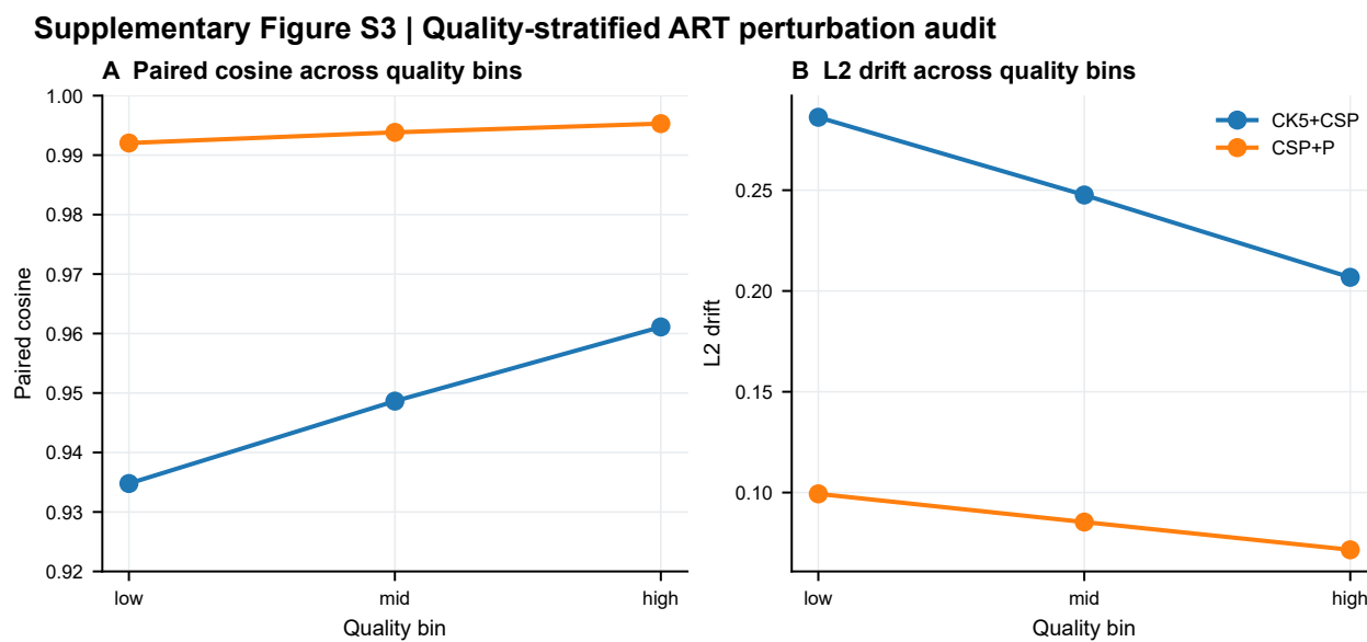
Figure S3 Quality-stratified ART perturbation audit.
