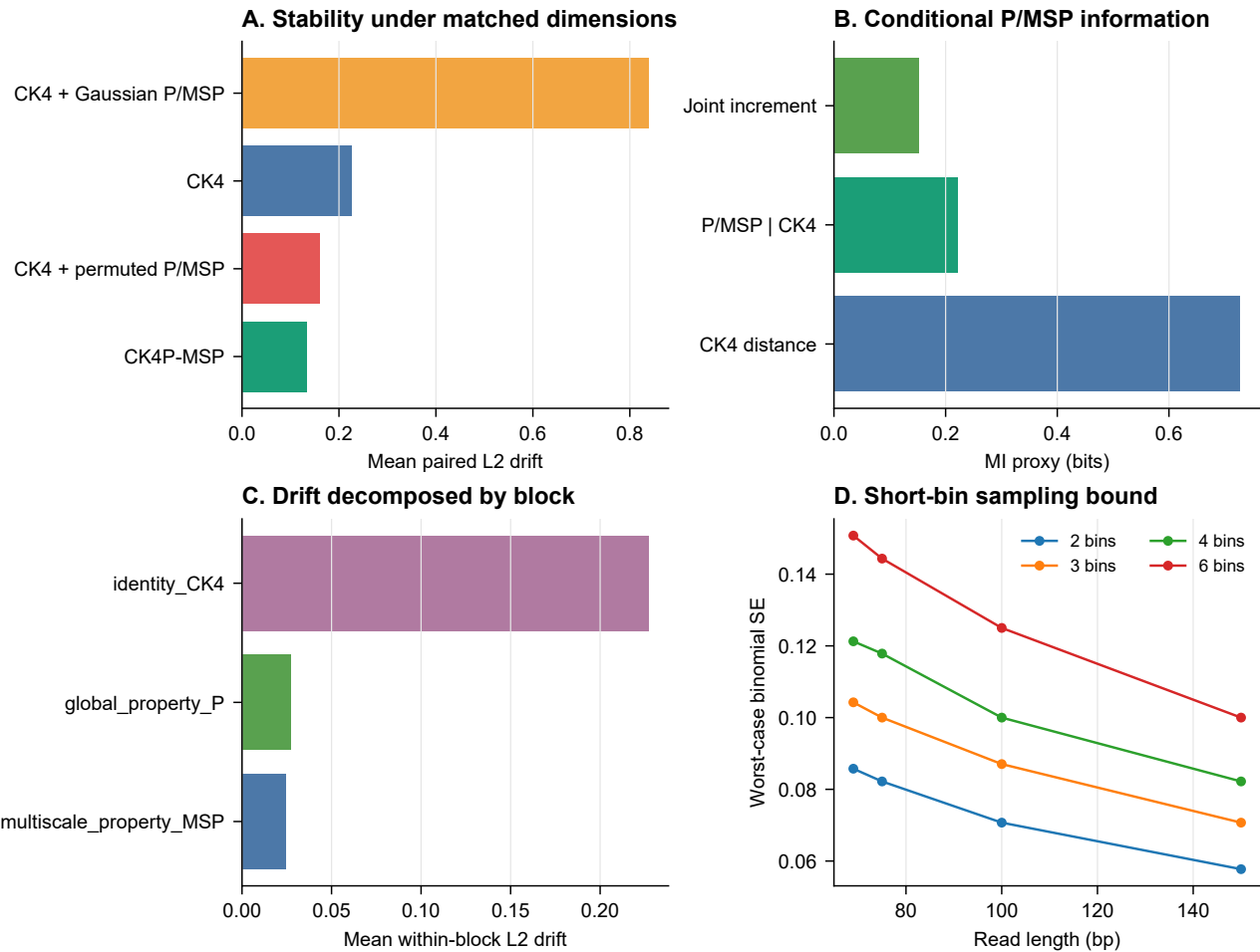
Figure S5 P-channel counterfactual and short-bin reliability audit.
