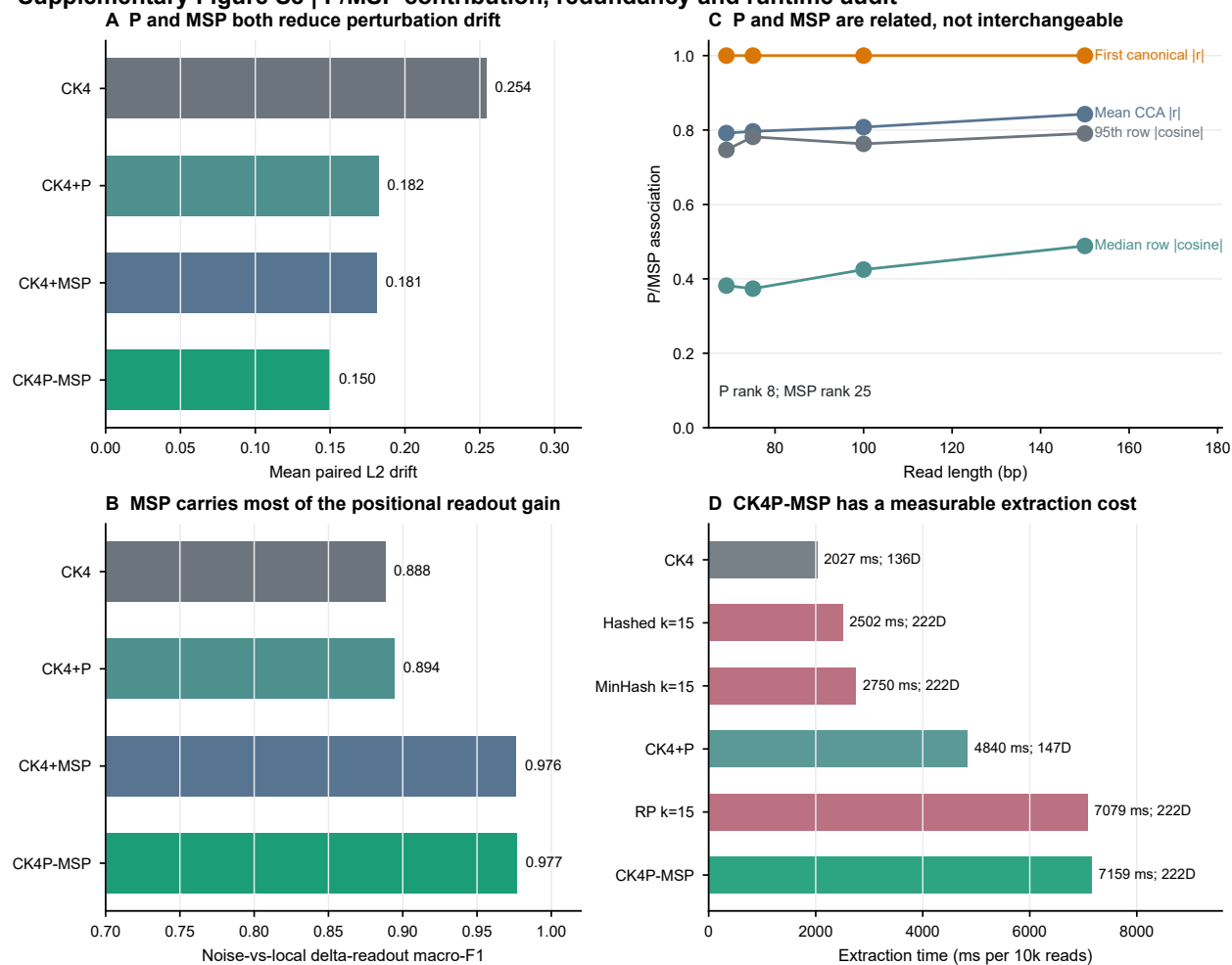
Figure S8 P/MSP contribution, redundancy and runtime audit.
