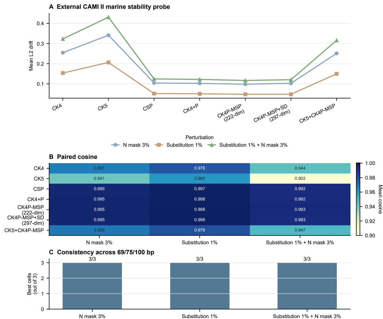
Figure S10 CAMI II marine anonymous-read stability probe.
