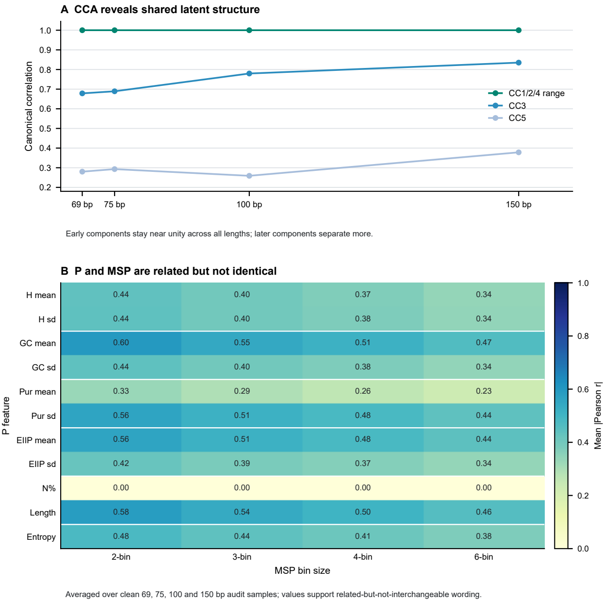
Figure S9 P/MSP relation audit.
