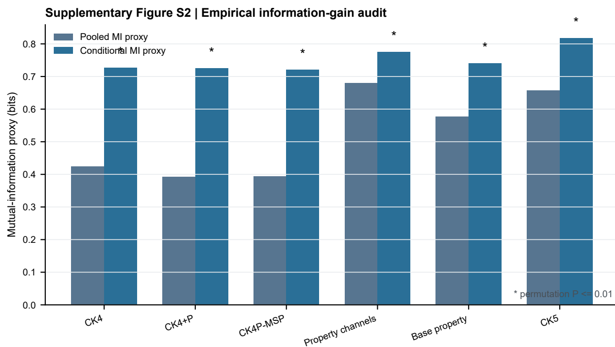
Figure S2 Empirical MI and conditional-MI audit.
