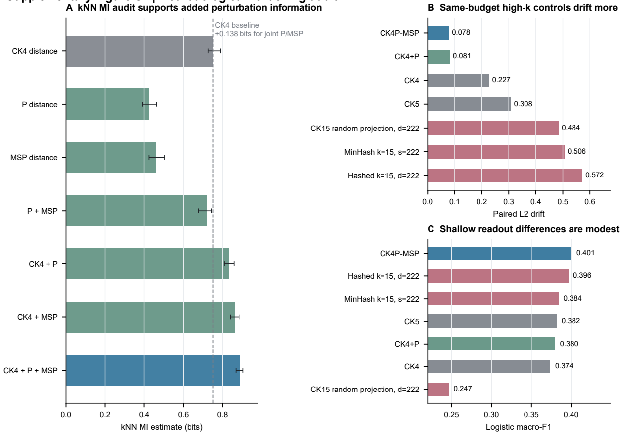
Figure S7 kNN MI robustness and dimension-matched high-k compressed baseline audit.
