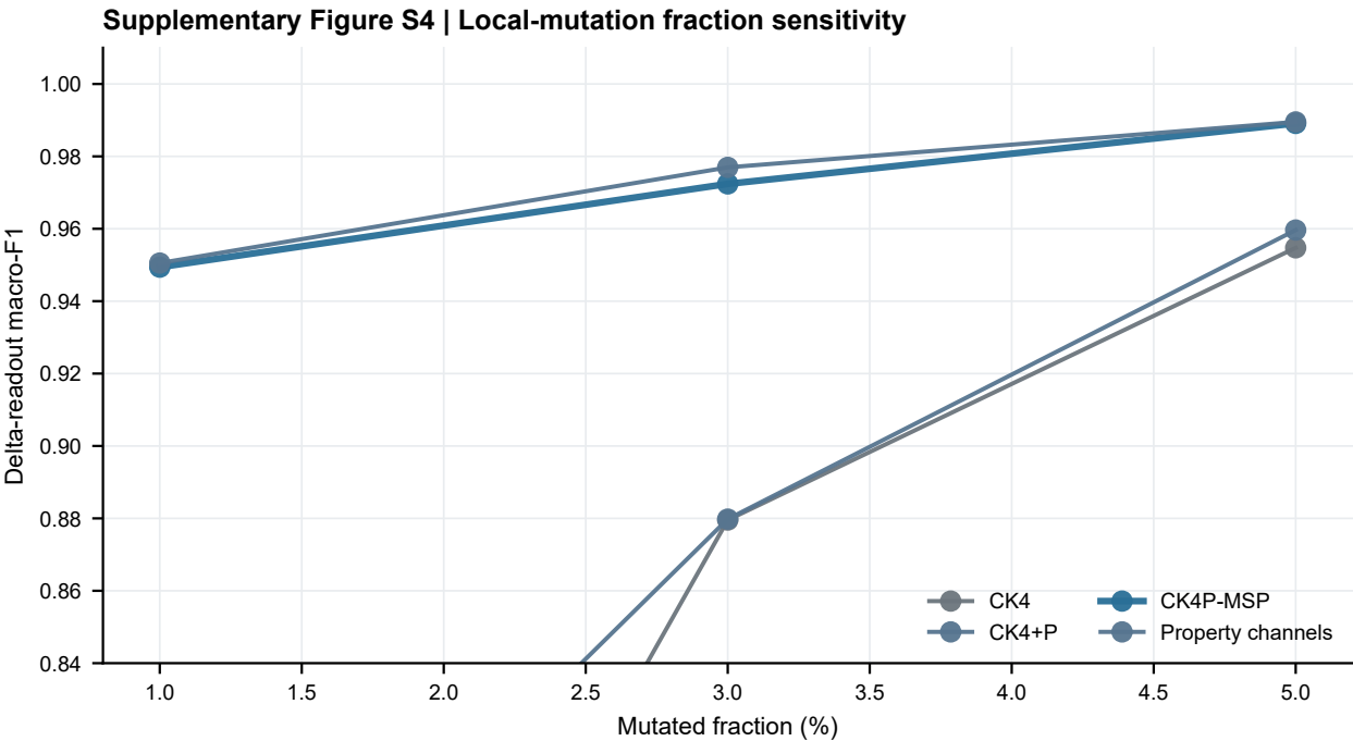
Figure S4 Local mutation-fraction sweep.
