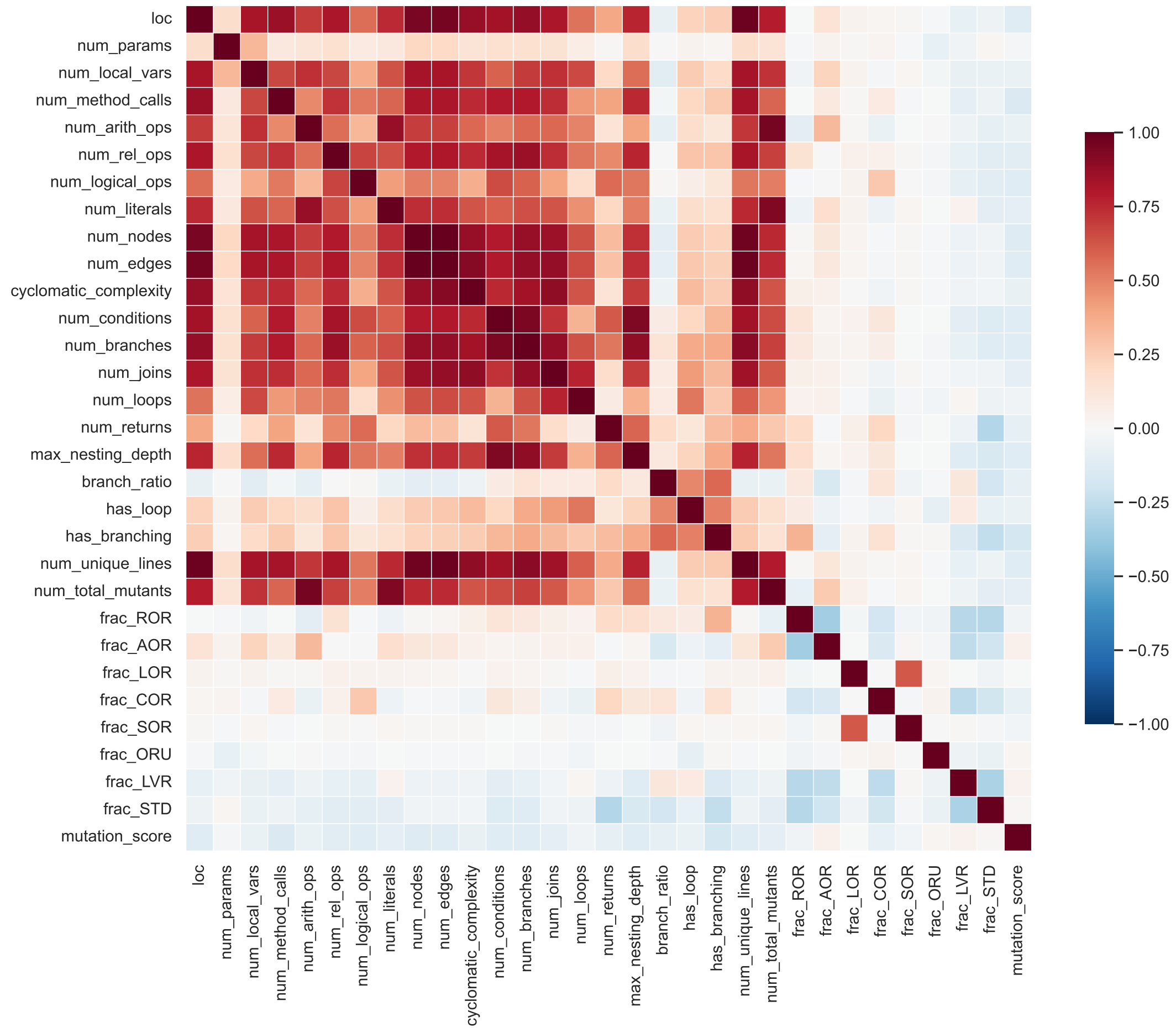
Pearson correlation matrix
