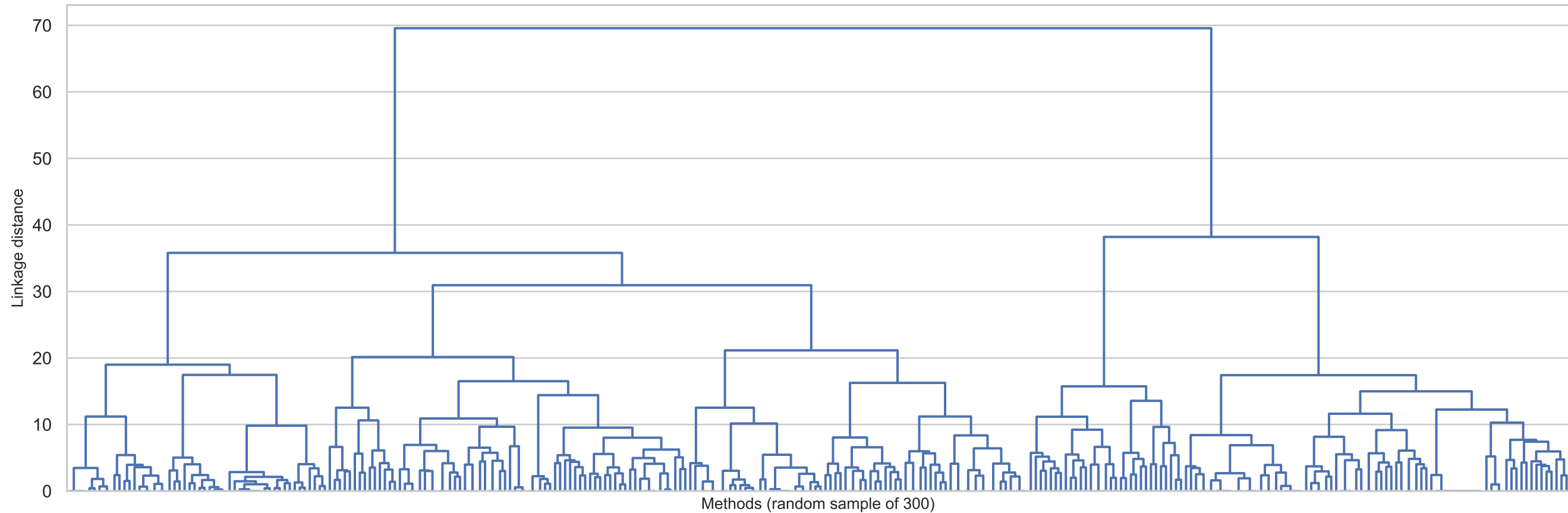
Hierarchical clustering dendrogram (Ward linkage)
