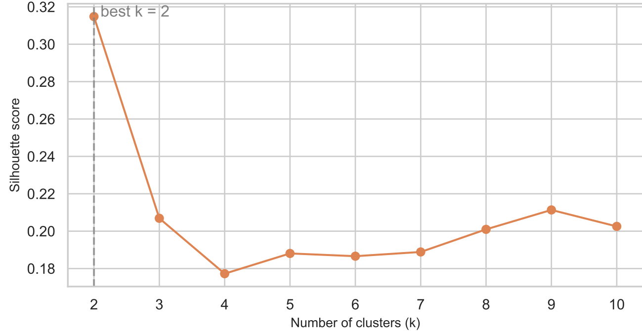
Silhouette analysis
