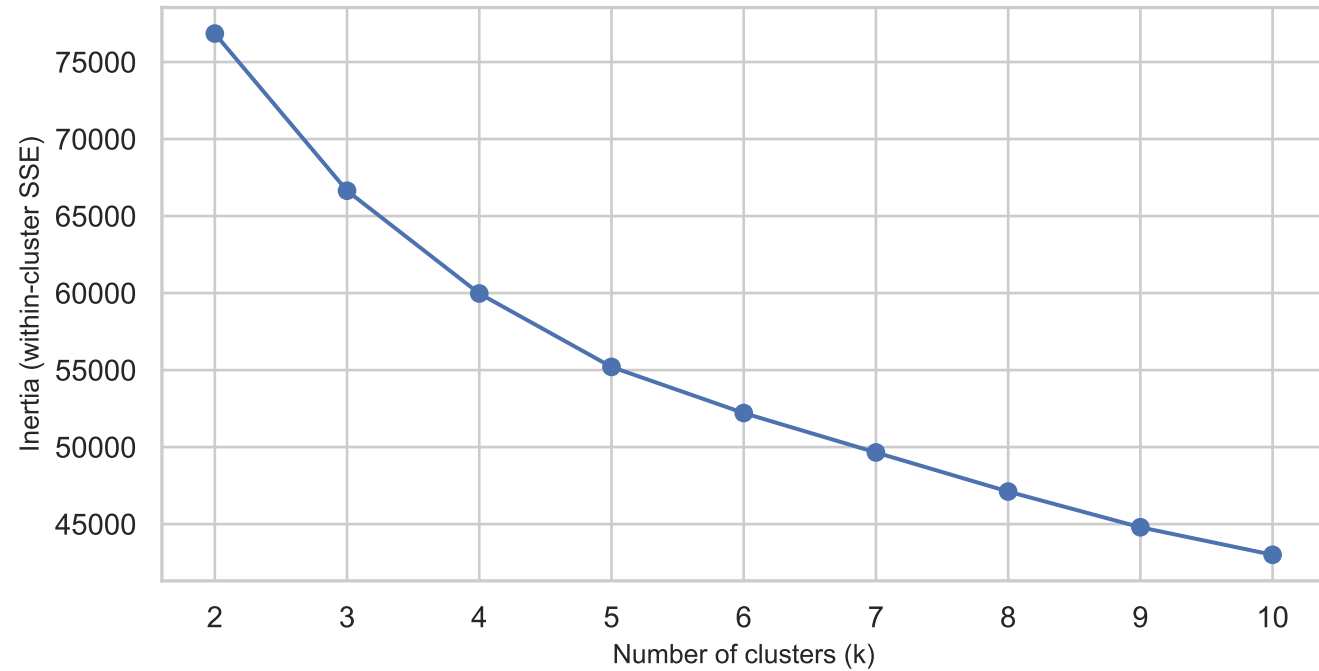
Elbow method
