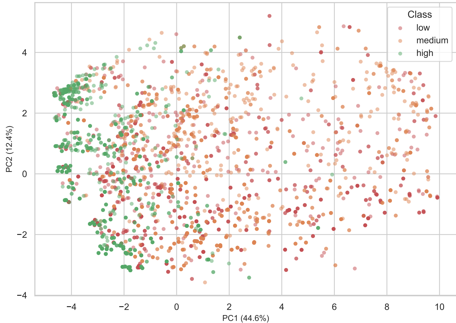
PCA 2D projection, colored by testability class
