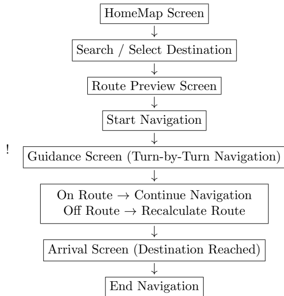
Figure 2: User Interface Flow of EagleNav
