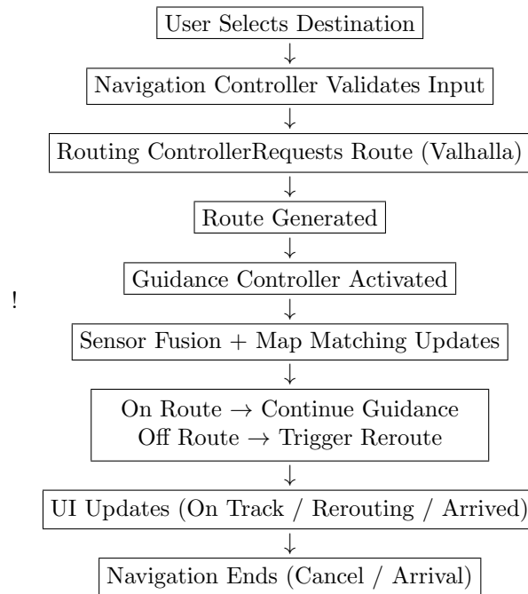
Figure 1: Compact Navigation Workflow
