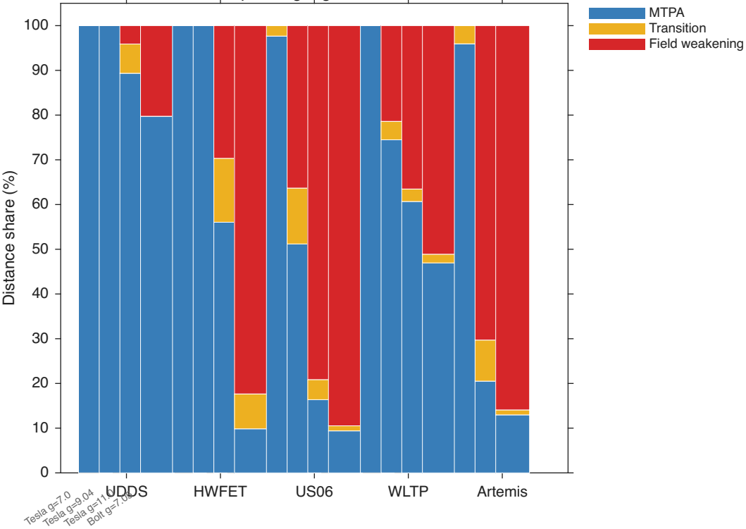
Motor operating regime distribution
