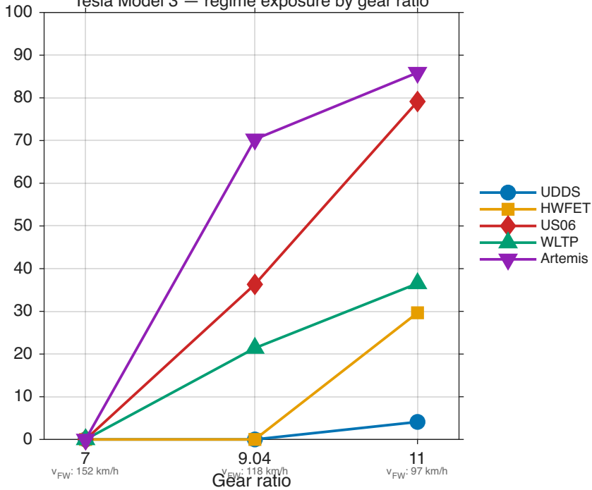
Tesla Model 3 — regime exposure by gear ratio
