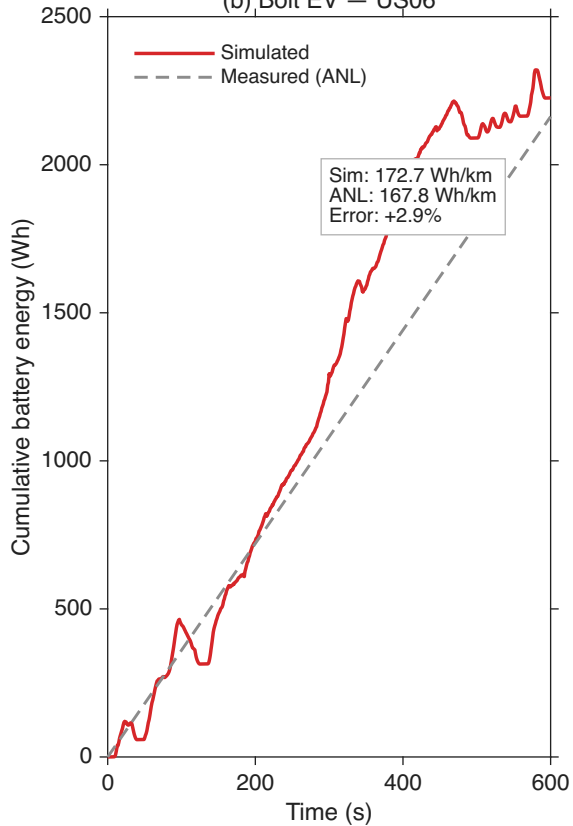
(b) Bolt EV — US06
