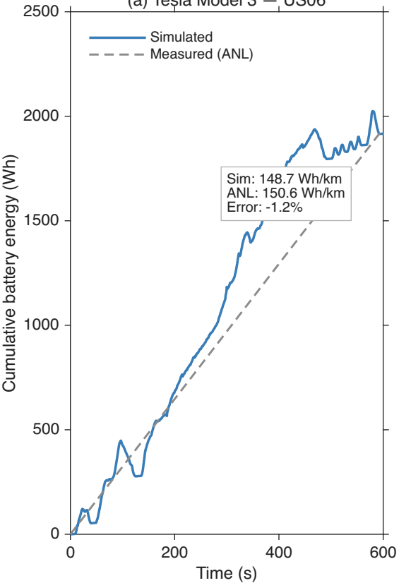
(a) Tesla Model 3 — US06
