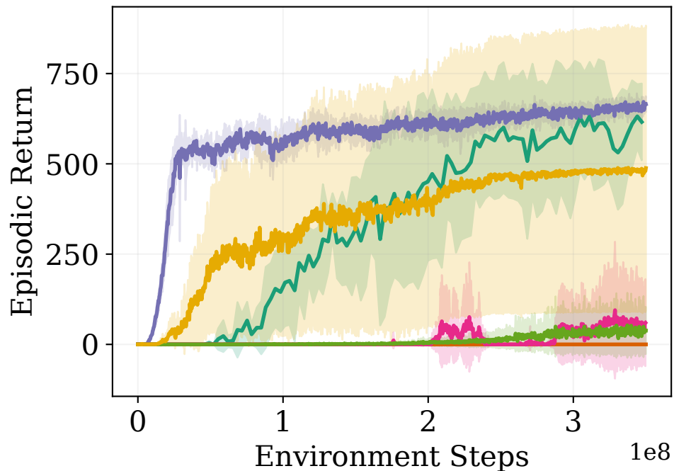
Ant u maze
