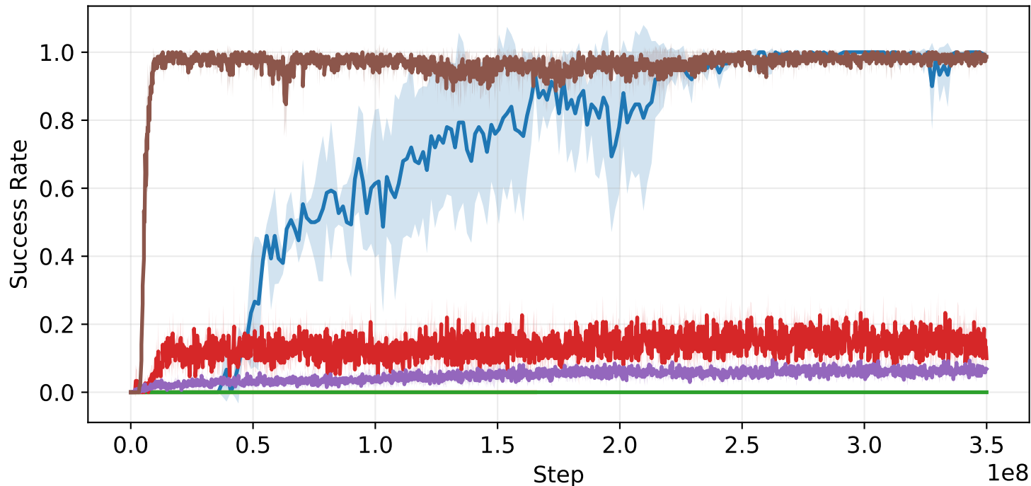
Ant-u-maze-single-goal
