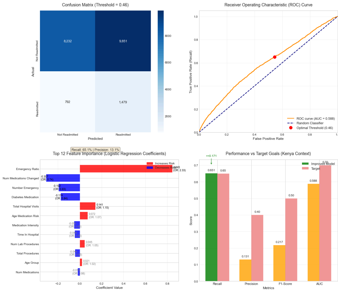
Improved Logistic Regression Model Evaluation
