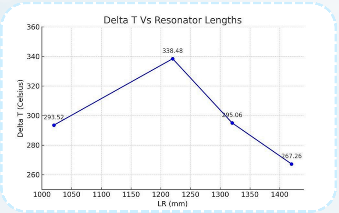
Delta T vs Resonator Lengths Graph for T-4, T-8,T-10 and T-12
