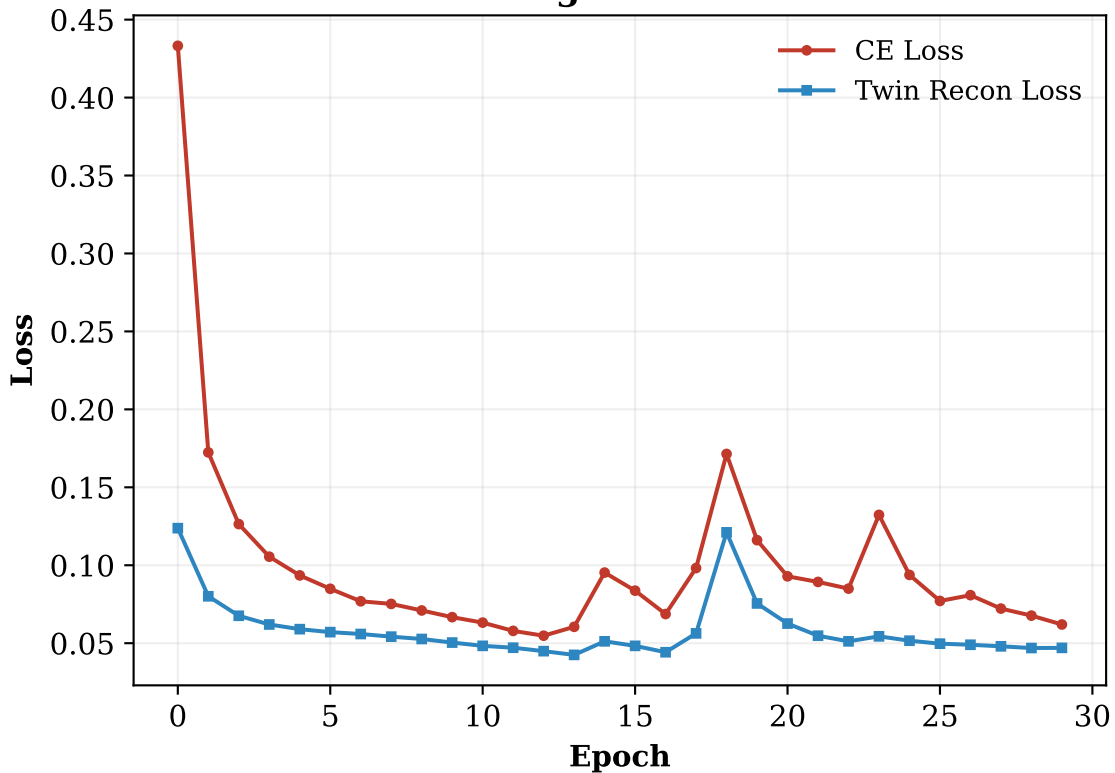
Training Loss Curves
