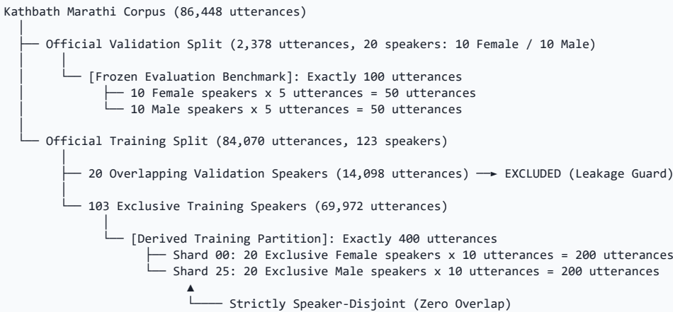
Figure 2: Dataset Partitioning and Leakage-Guarded Sampling Workflow
