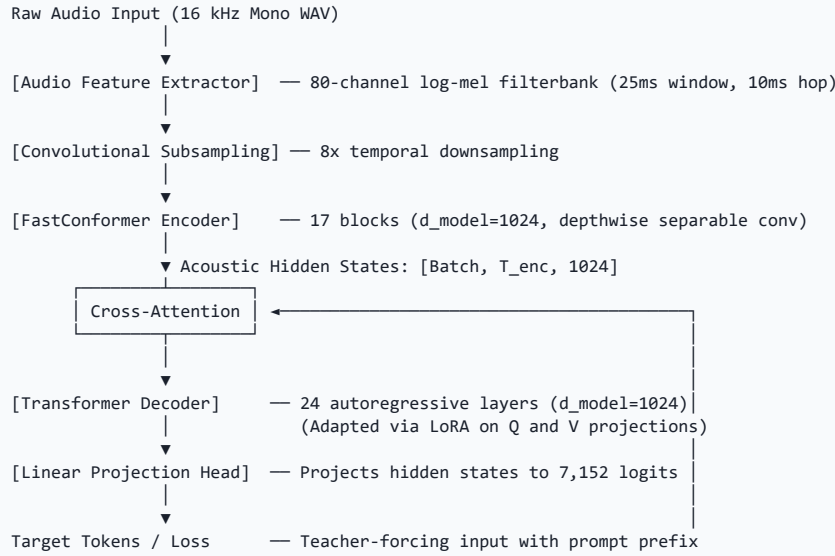
Figure 1: Architectural Topology of Indic-Canary 1.22B Foundation Model
