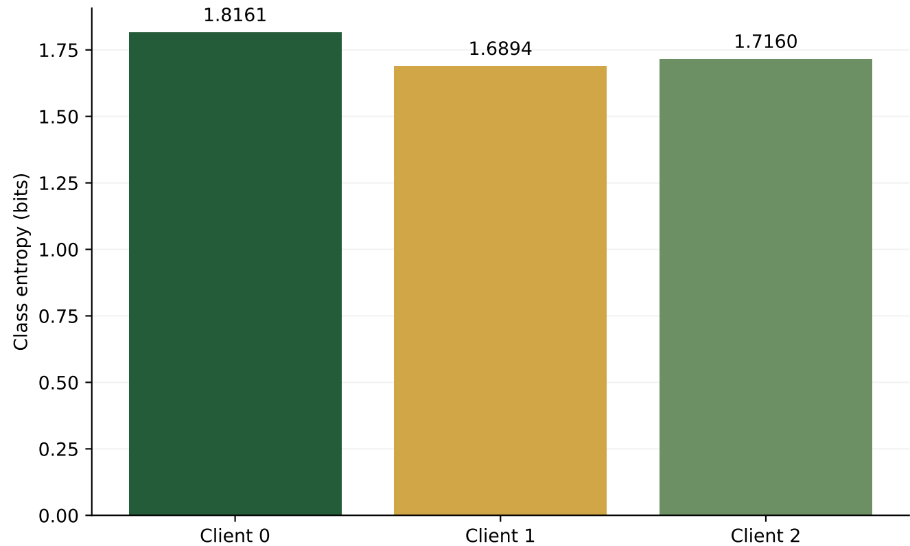
Rice client class entropy ( \alpha=0.1 )
