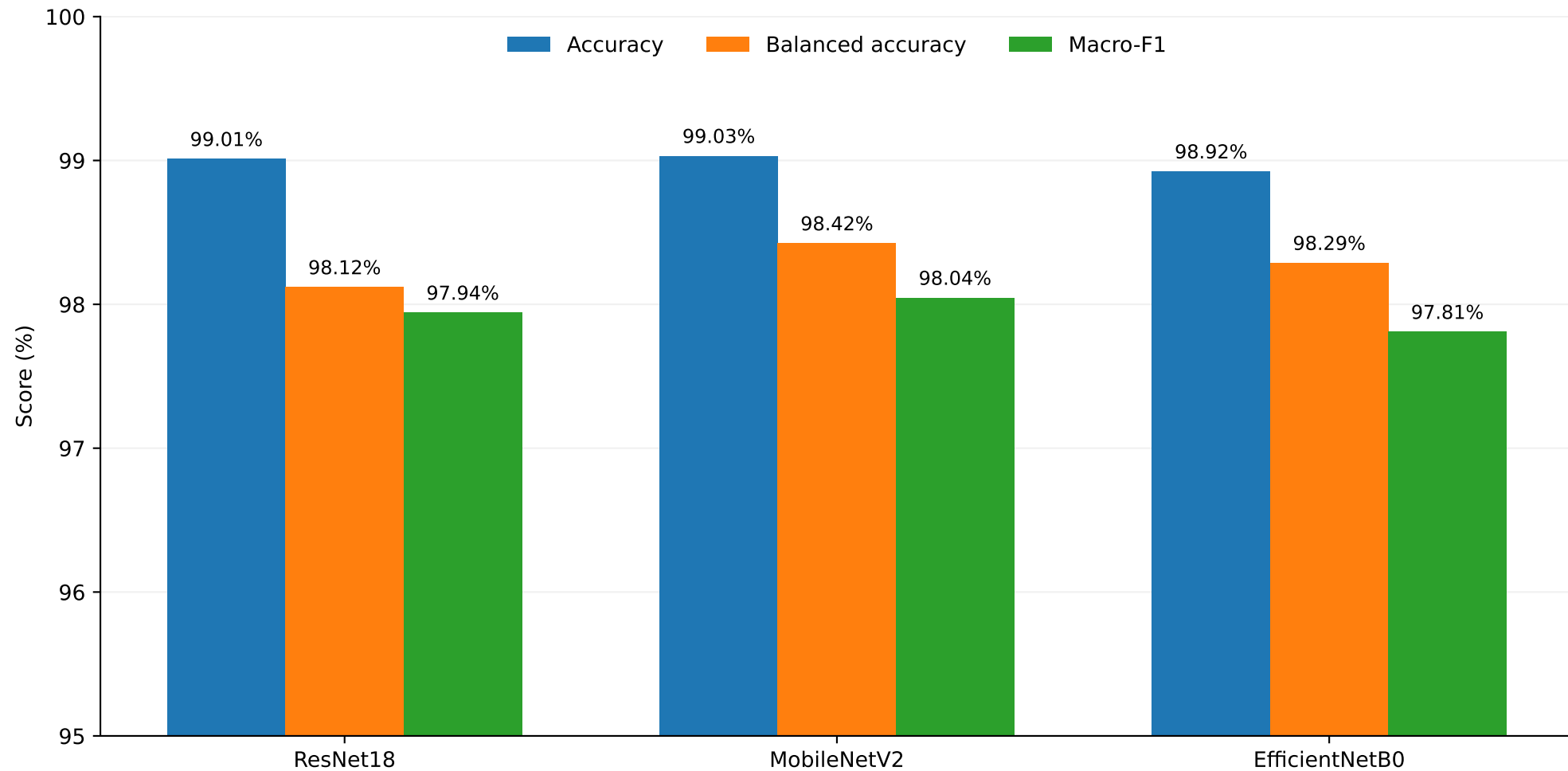
Centralized rice architecture comparison on the test set
