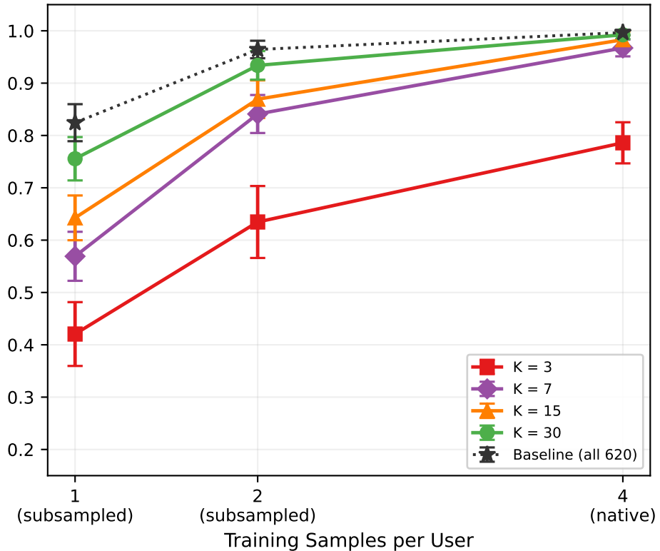
(b) Scenario 3.2: data volume effect
