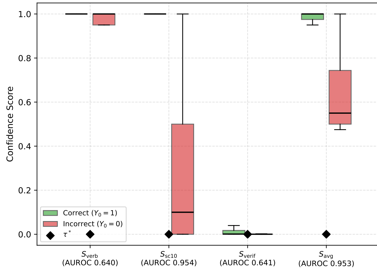
Qwen2.5-7B-Instruct on GSM8K
