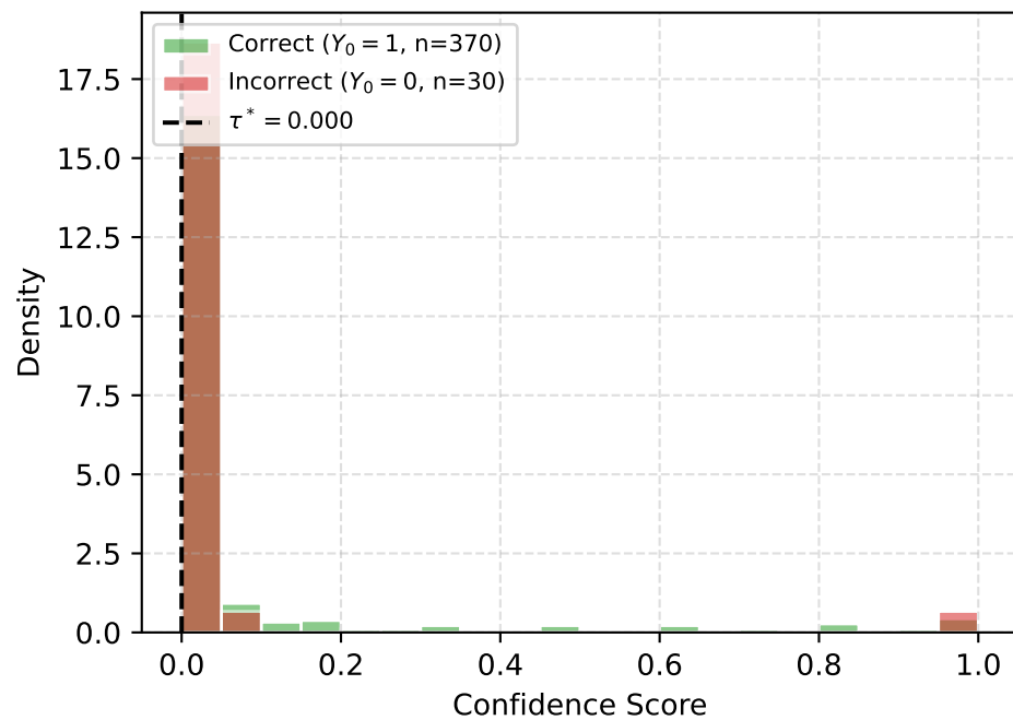
S_{\text{verif}} (AUROC = 0.641)
