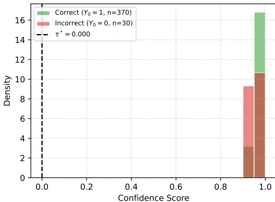
S_{\text{verif}} (AUROC = 0.641)
