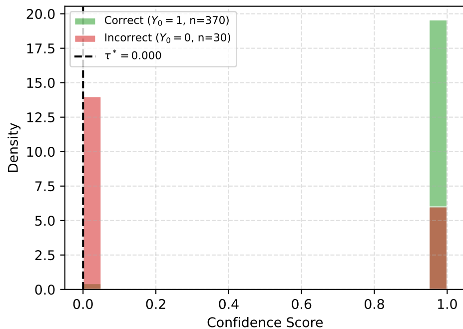
S_{\text{avg}} (AUROC = 0.840)
