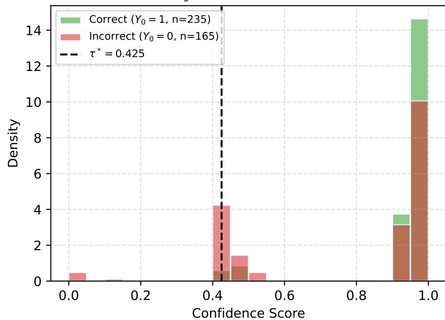
S_{\text{avg}} (AUROC = 0.662)
