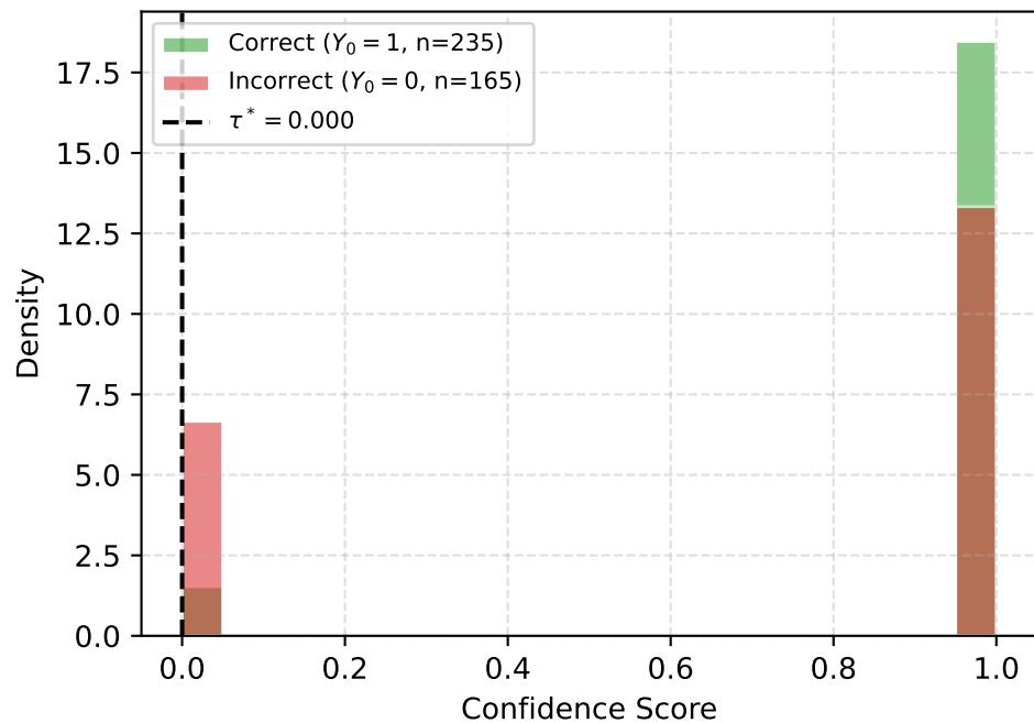
S_{\text{avg}} (AUROC = 0.662)
