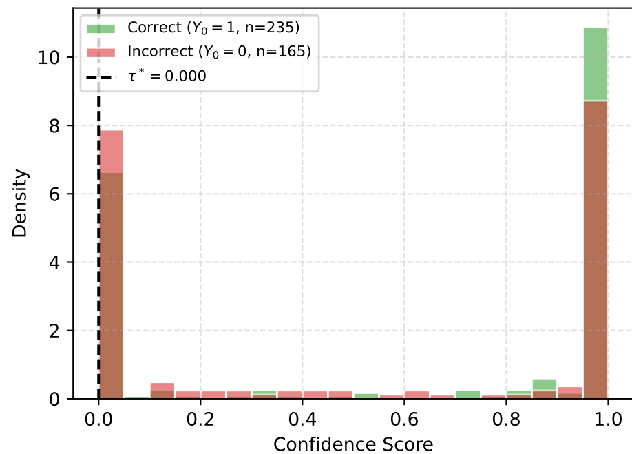
S_{\text{verif}} (AUROC = 0.577)
