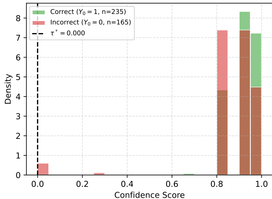
S_{\text{verif}} (AUROC = 0.577)
