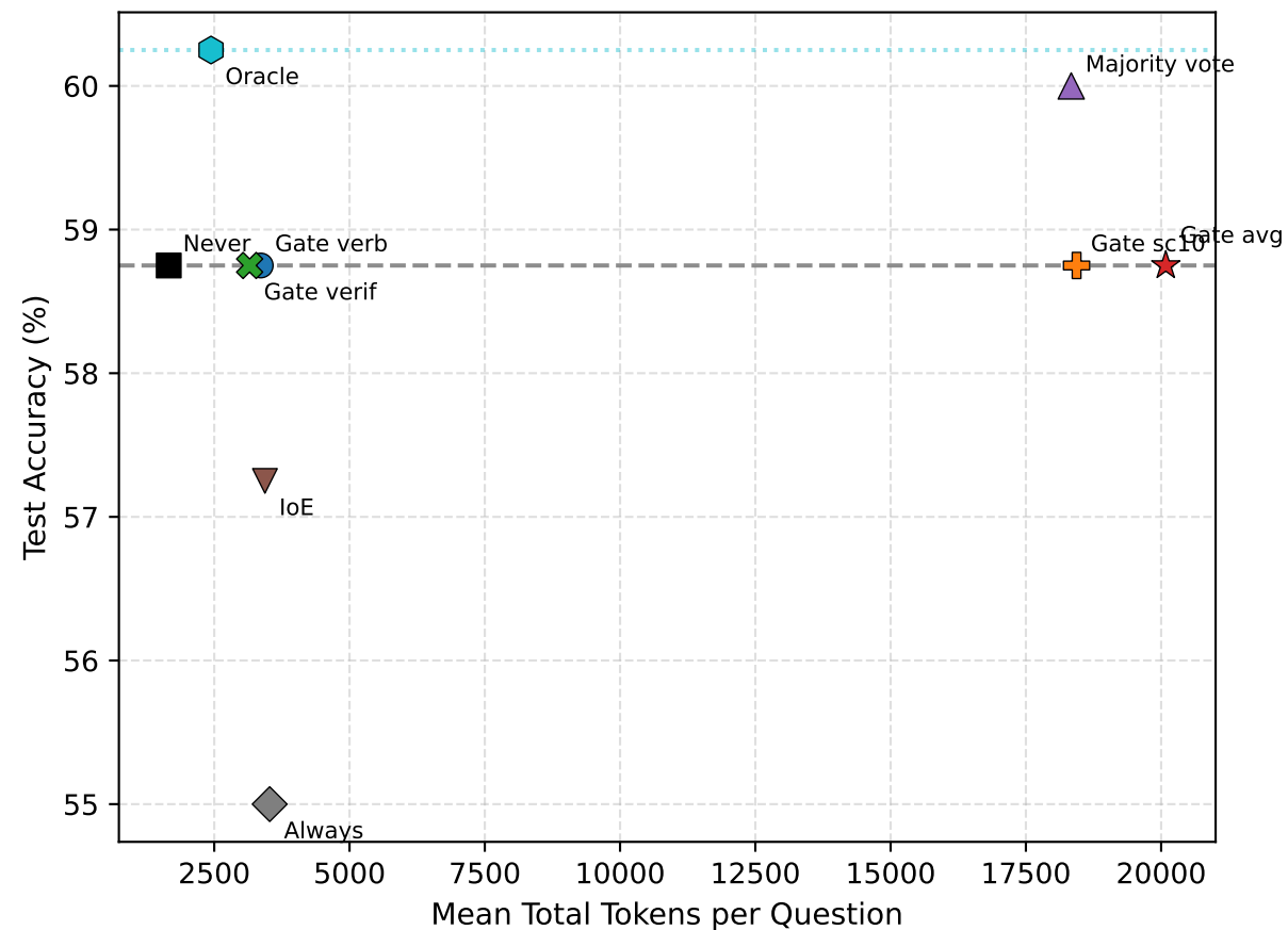
Qwen2.5-7B-Instruct on HOTPOTQA
