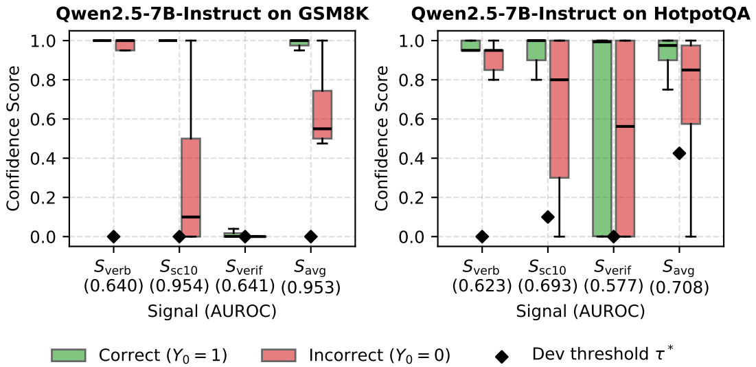
Figure 3: Distributions of confidence scores for correct ( Y_0 = 1 ) versus incorrect ( Y_0 = 0 ) initial answers across signals on GSM8K (left) and HotpotQA (right) for Qwen2.5-7B-Instruct. Diamonds indicate the dev-selected threshold \tau^* .
