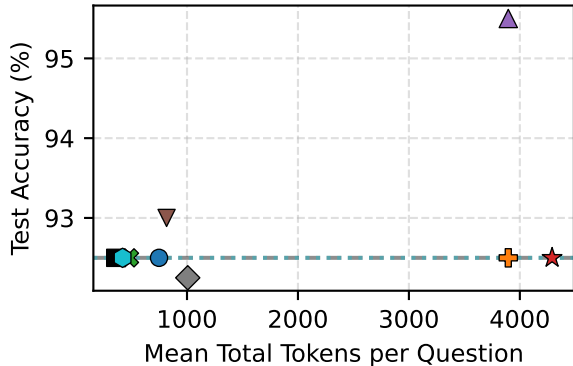
Qwen2.5-7B-Instruct on GSM8K
