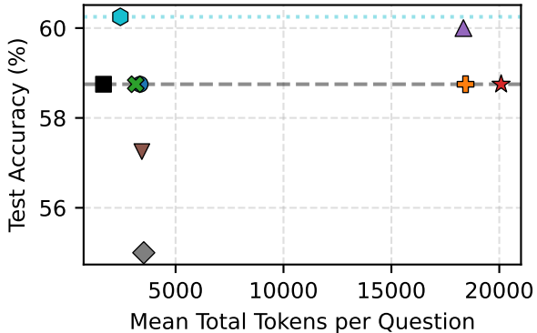
Qwen2.5-7B-Instruct on HotpotQA
