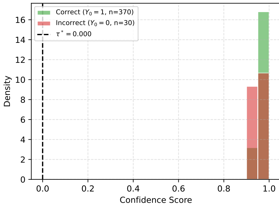
S_{\text{verif}} (AUROC = 0.641)
