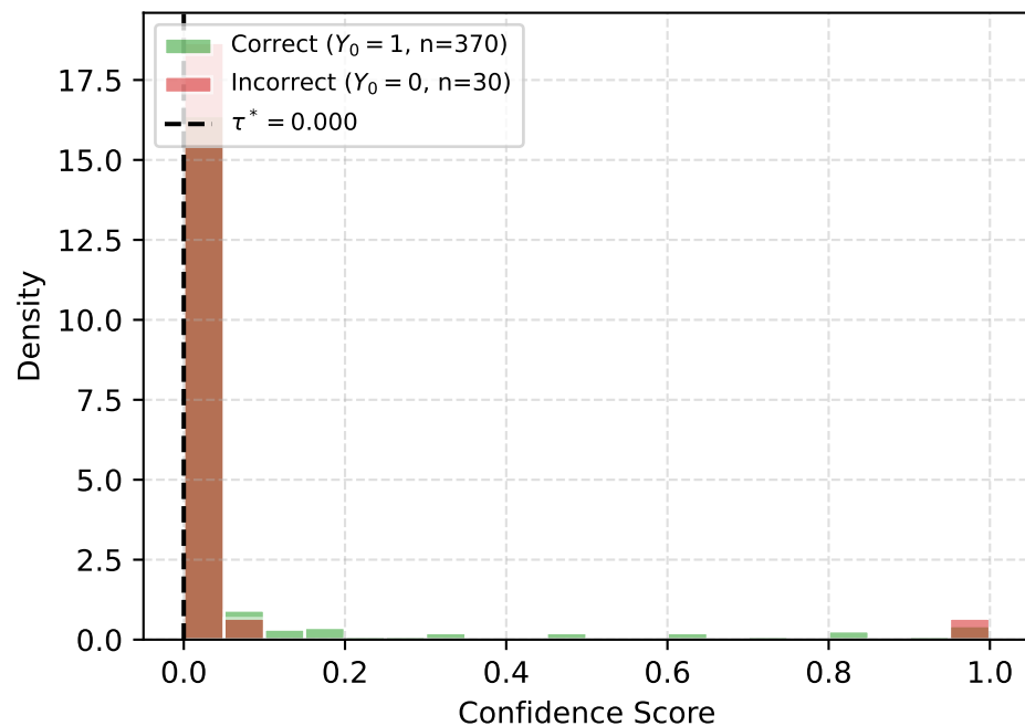
S_{\text{verif}} (AUROC = 0.641)
