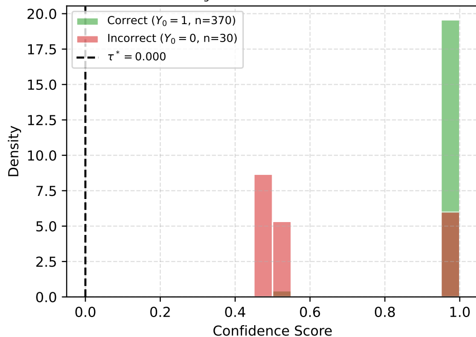
S_{\text{avg}} (AUROC = 0.840)
