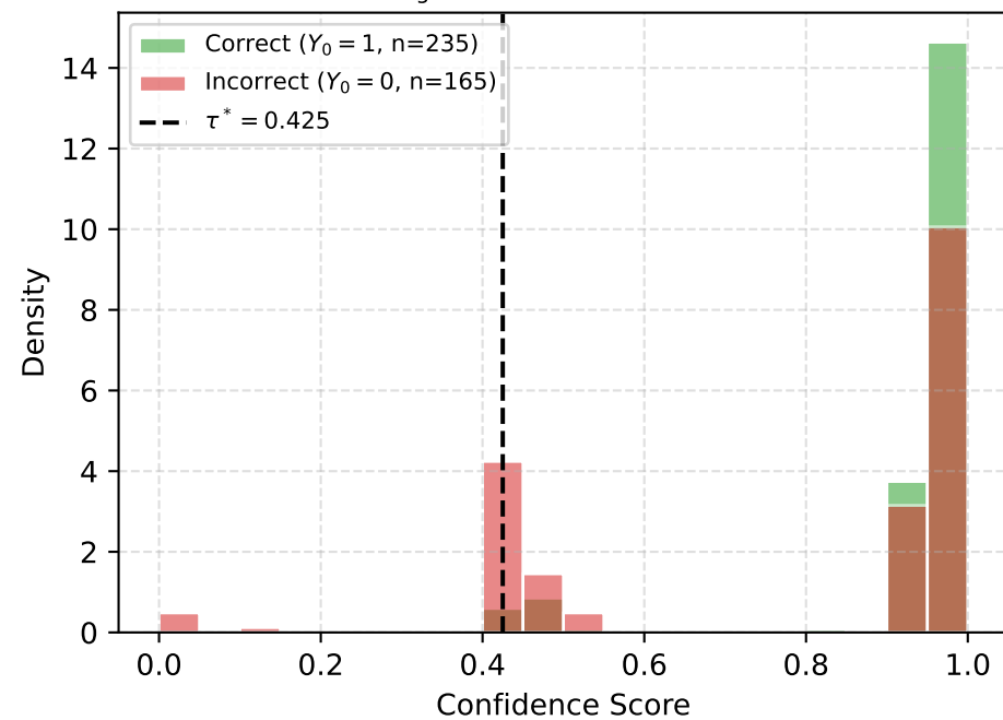
S_{\text{avg}} (AUROC = 0.662)
