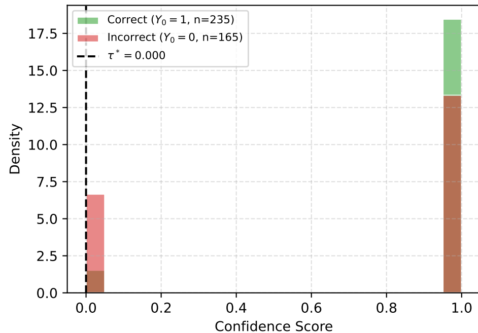
S_{\text{avg}} (AUROC = 0.662)
